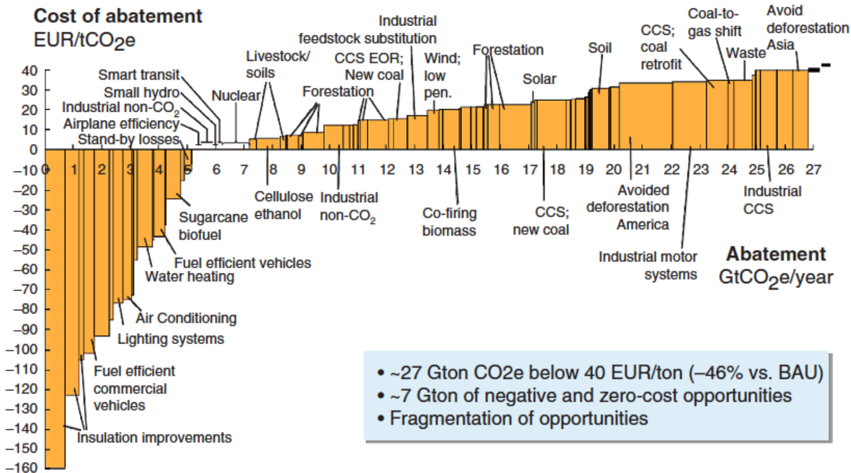
Figure 5. Estimates of worldwide potential for greenhouse gas emission reductions (billions of metric tons of CO 2 equivalents per year, GtCO 2 e/year) at a mitigation cost of less than 40 euros per ton. 11 CCS EOR is carbon dioxide capture CO 2 -enhanced oil recovery. BAU is “business as usual.”
