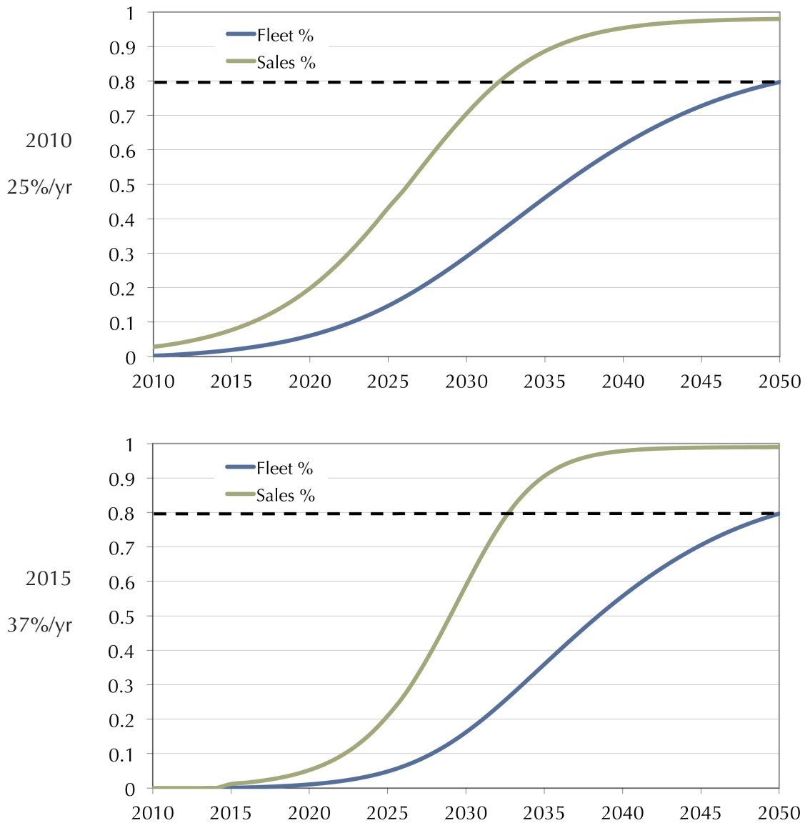
Figure 1. Introduction year and annual sales growth rate for hypothetical advanced vehicle introduction to reach 80% fleet share in 2050
