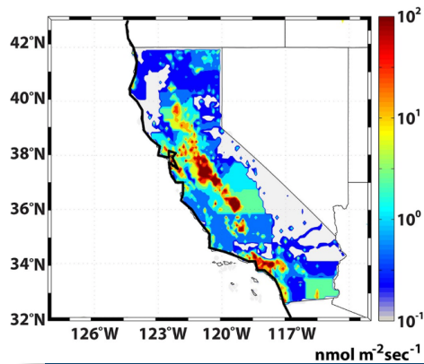
FIGURE 2: Modeled methane emissions refined using AJAX trace gas measurements over the San Joaquin Valley
