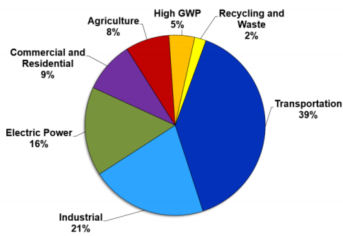
FIGURE 1: GHG Emissions by Economic Sector
